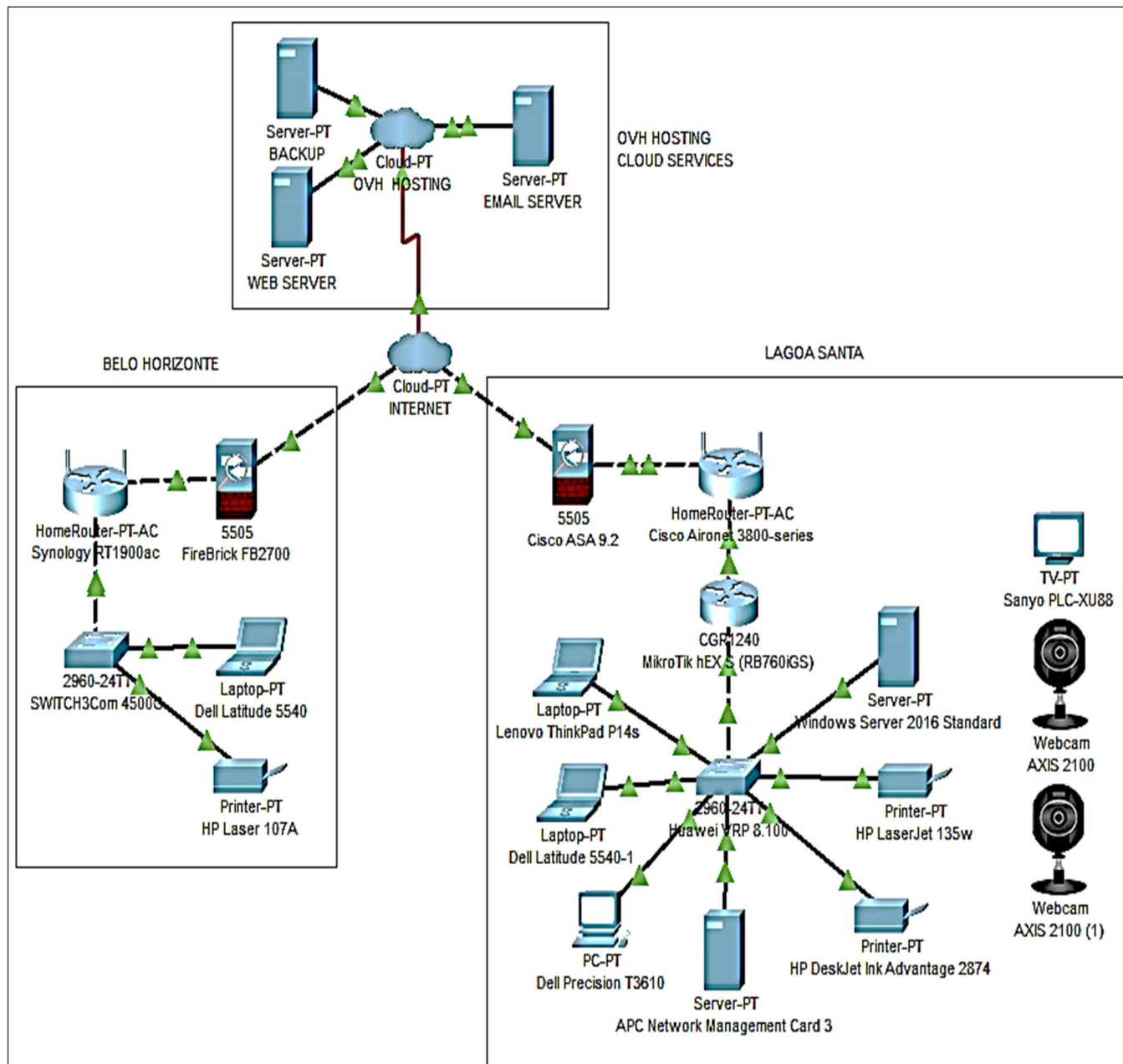
Diagrama elaborado com PACKET TRACER
